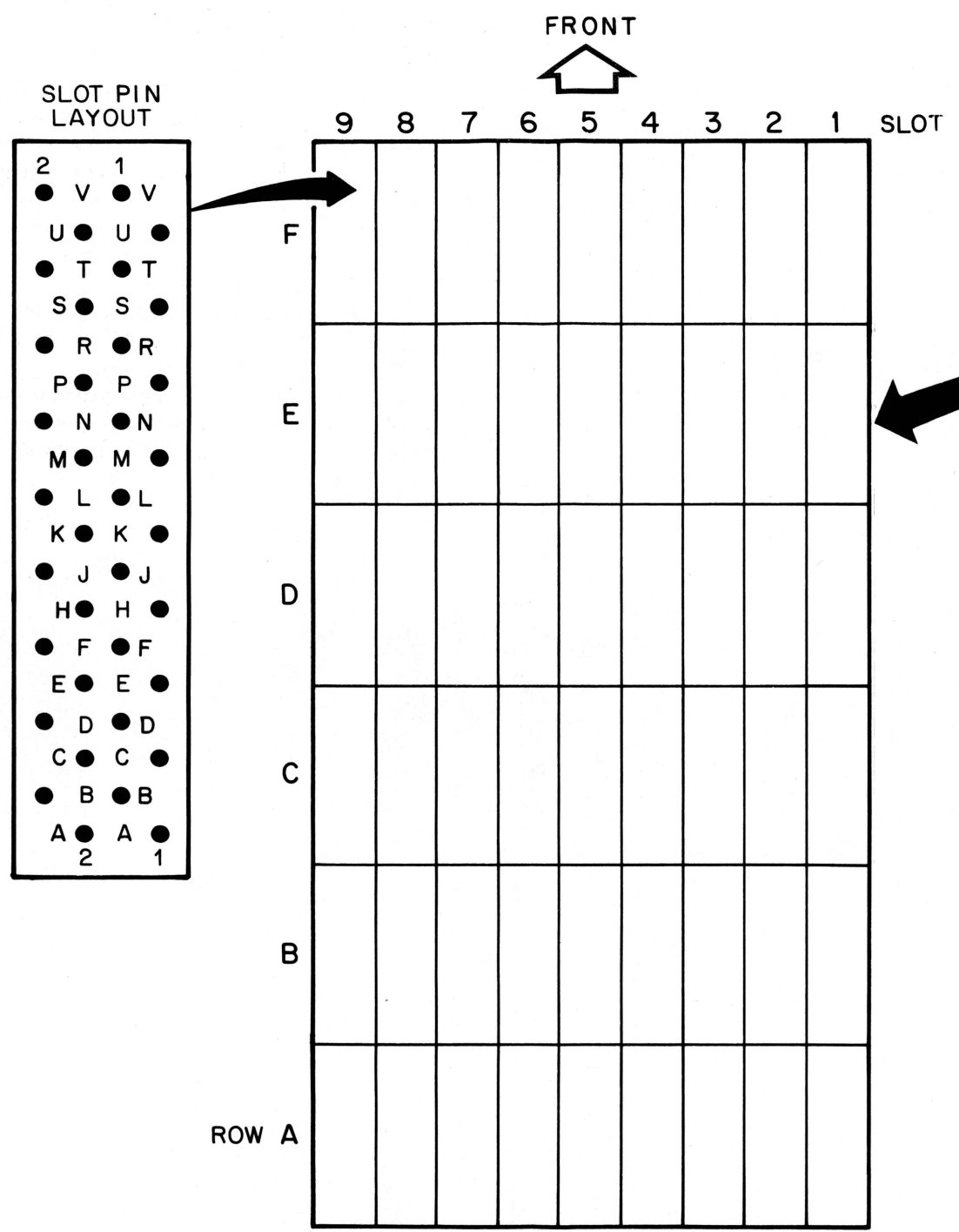
VIEW FROM WIRE WRAP PIN SIDE. COMPUTER IN MAINTENANCE POSITION
