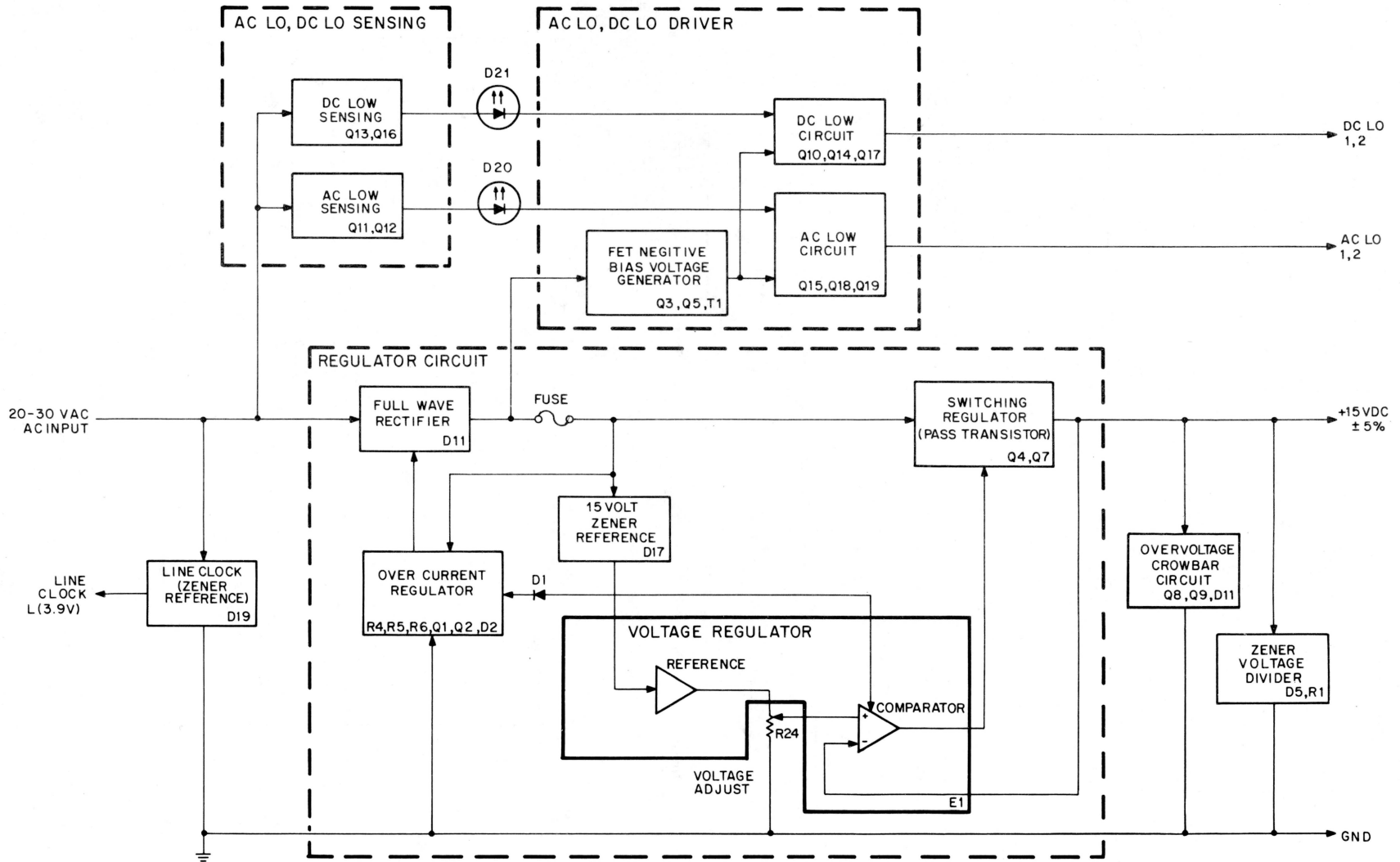
Figure 3-6 5411086 Block Diagram
