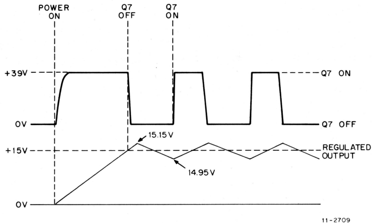
Figure 3-7 5411086 Regulator Waveforms
