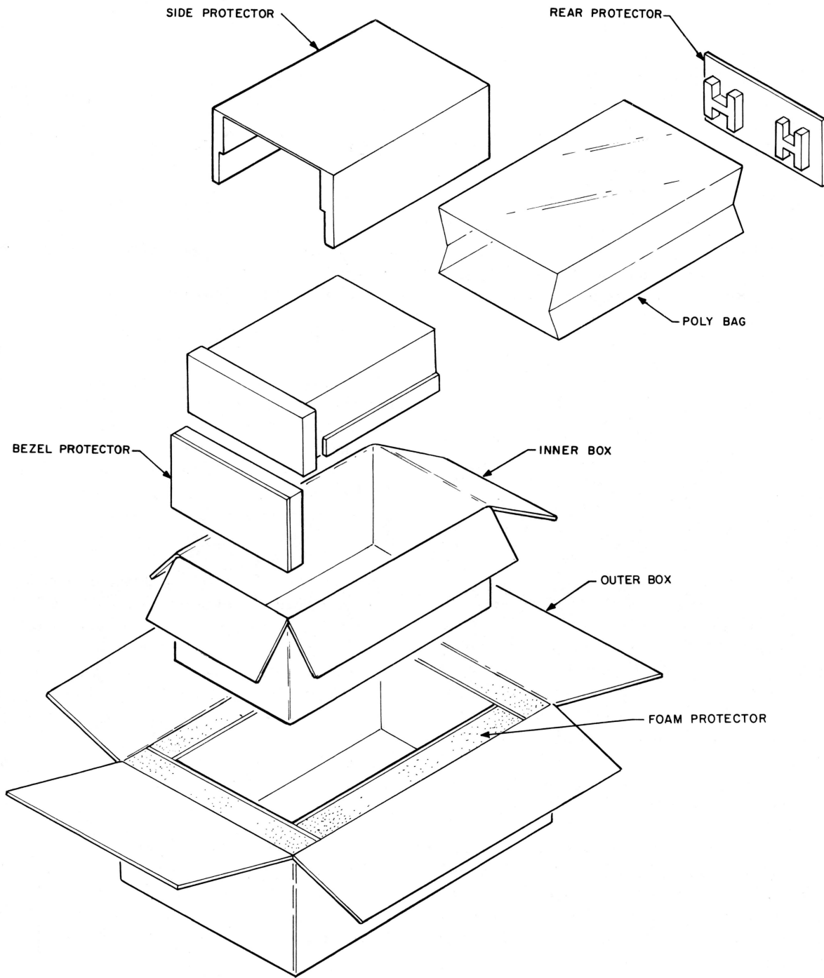
Figure 5-1 BA11-K Packaging
