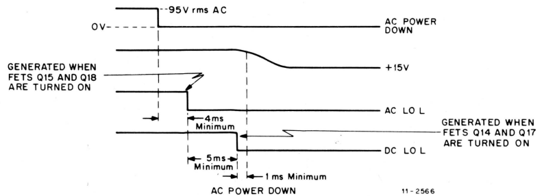
Figure 3-8 5411086 Power Up and Power Down
