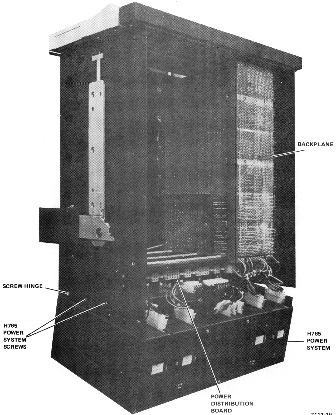
Figure 4-4 H765 Power System Access (Maintenance Position)
