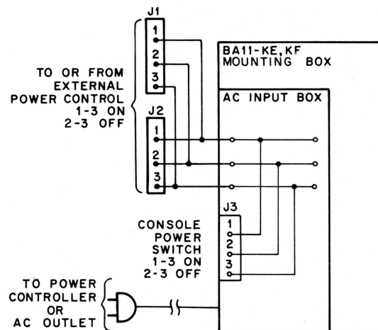
Figure 5-3 Power Control
