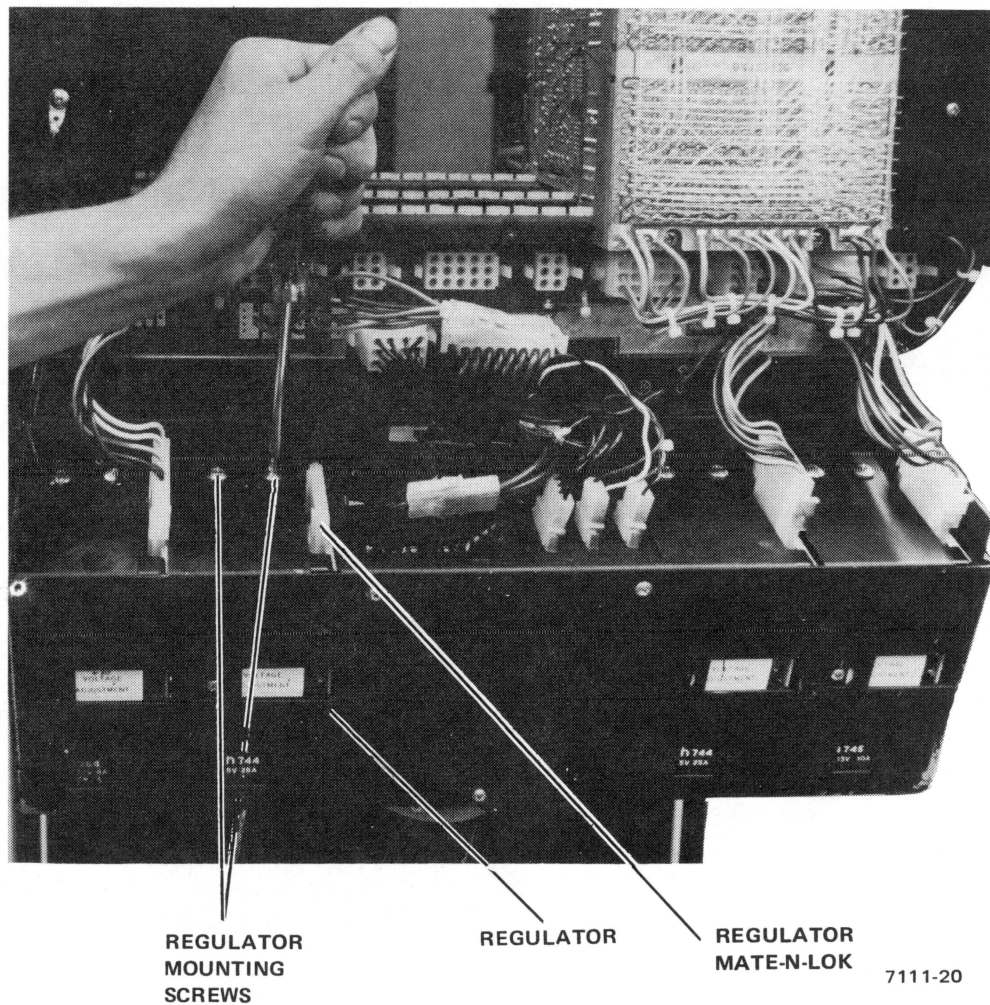
Figure 4-5 Regulator Removal
