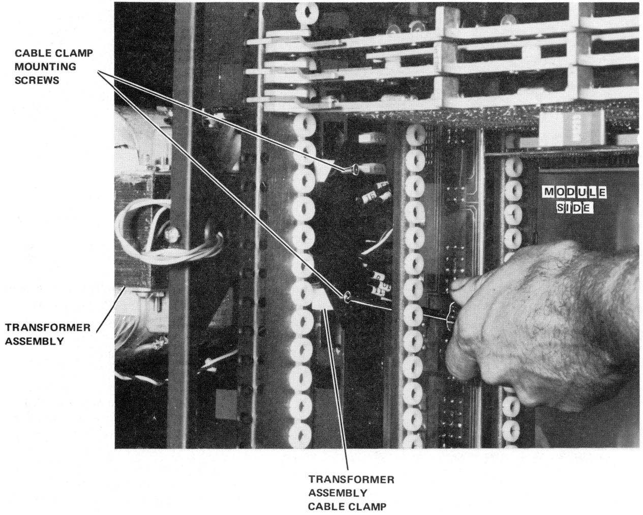
Figure 4-9 Transformer Assembly Removal (Sheet 2 of 2)
