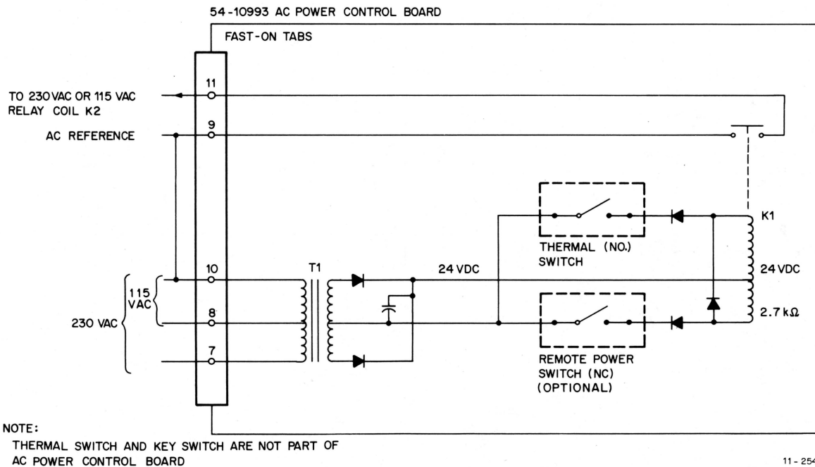
Figure 3-5 Power Control Simplified Diagram
