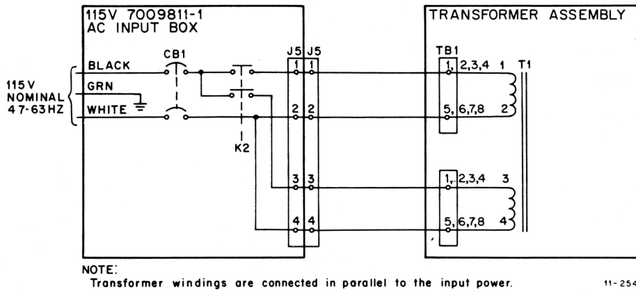
Figure 3-3 115 V Power Configuration
