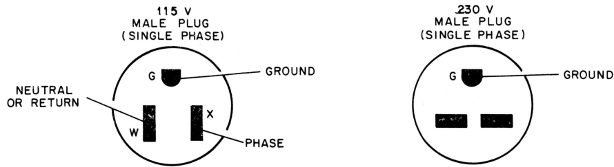
CONNECTOR SPECIFICATIONS
