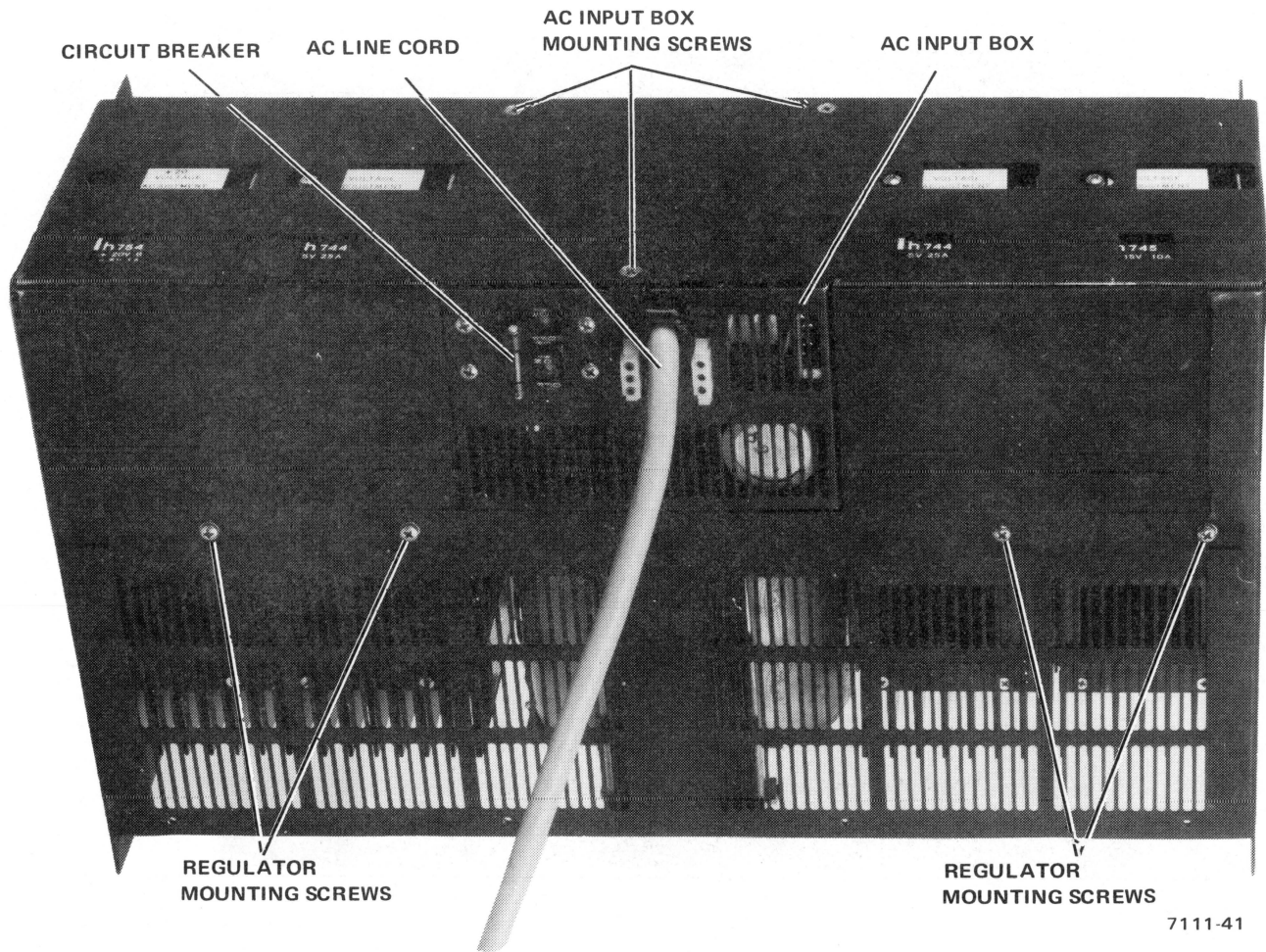
Figure 4-6 H765 Power System
