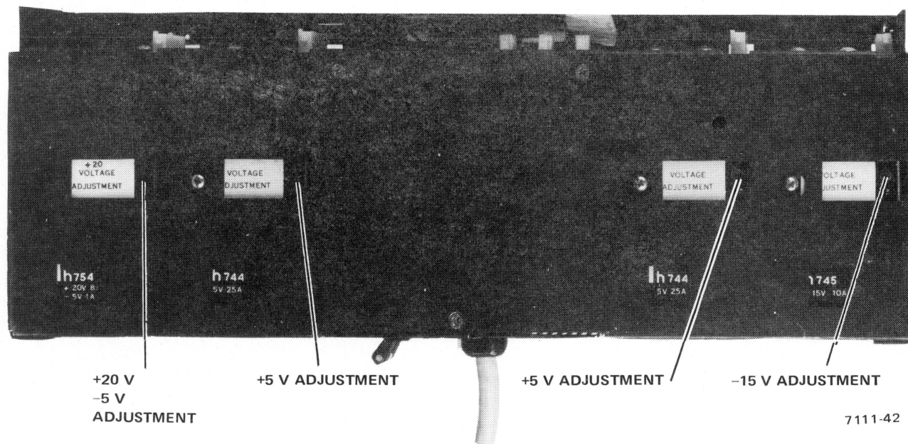
Figure 4-2 Regulator Adjustments
