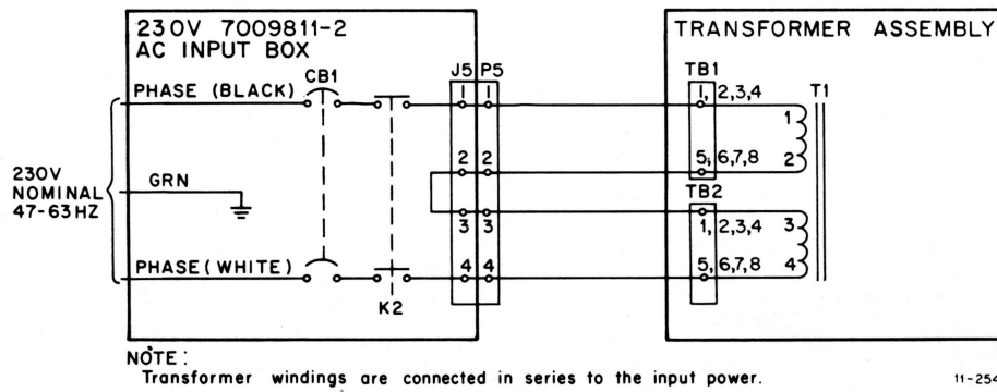
Figure 3-4 230 V Power Configuration
