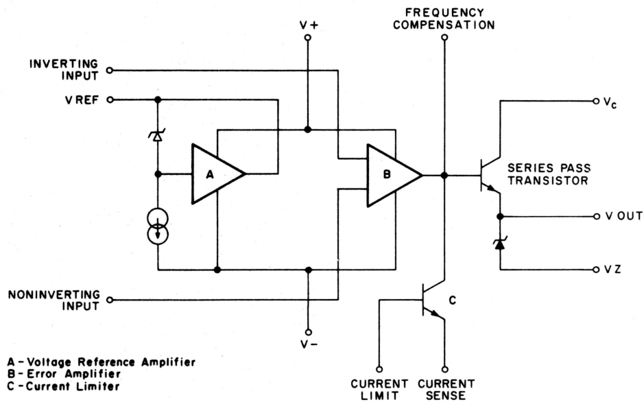
Simplified Schematic
