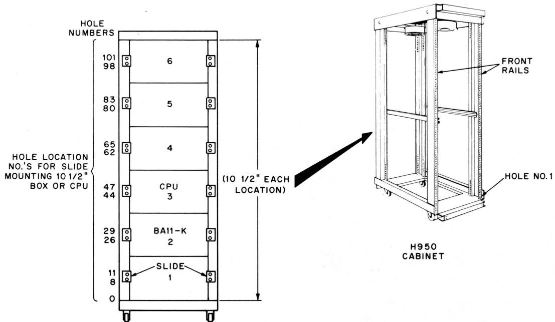
Figure 2-6 BA11-K and CPU Cabinet Mounting Specification
