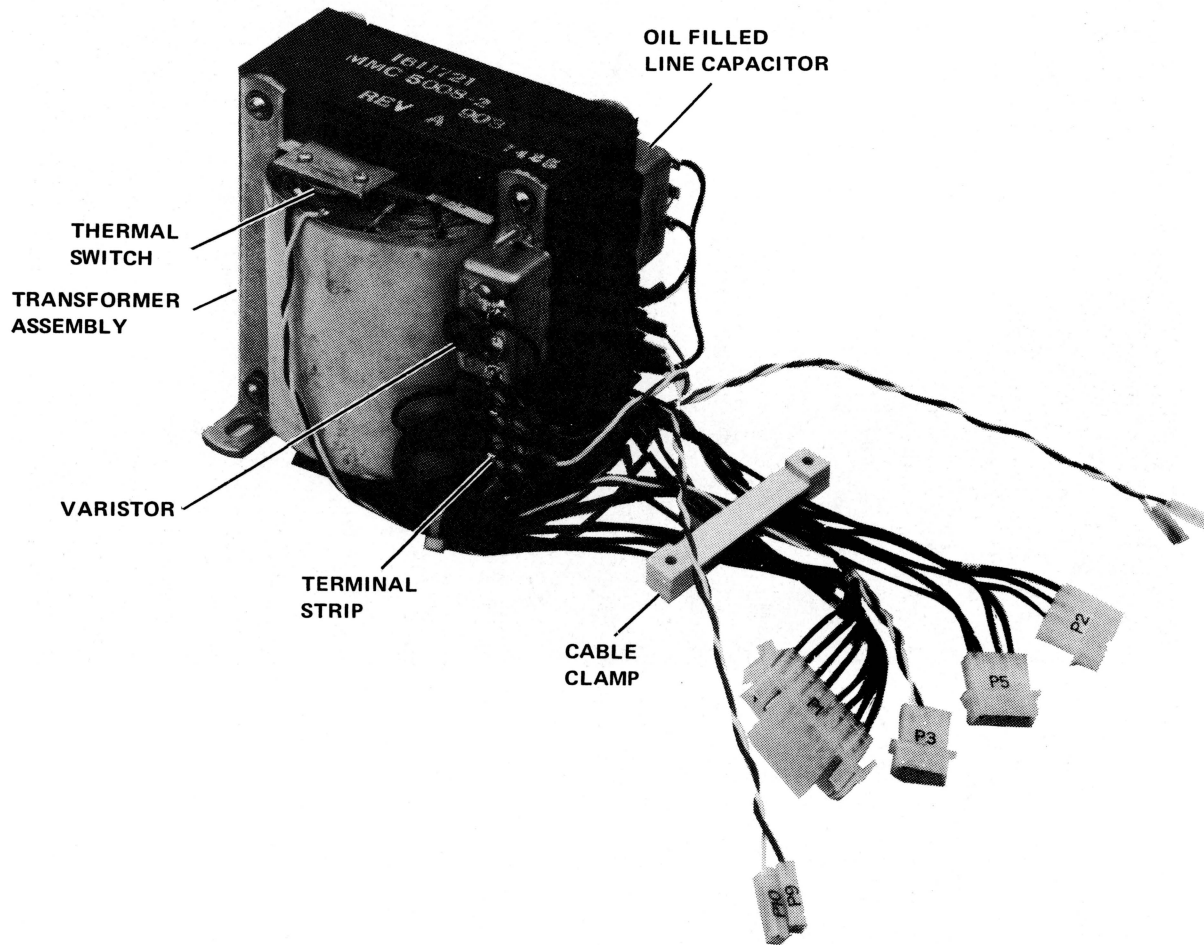
Figure 4-8 Transformer Assembly
