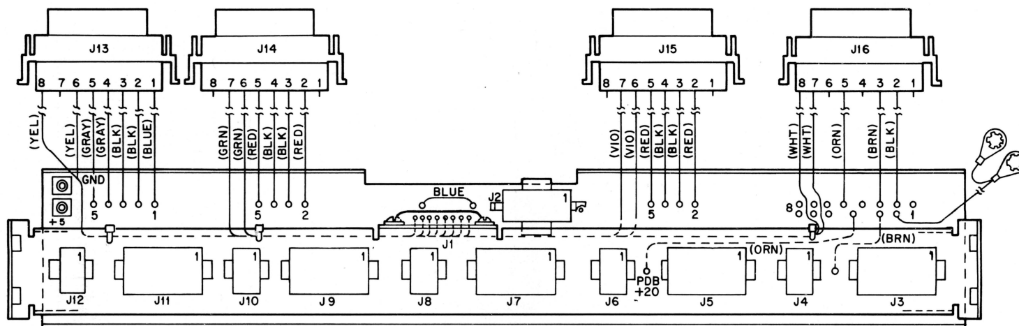
Figure 3-11 Power Distribution Board
