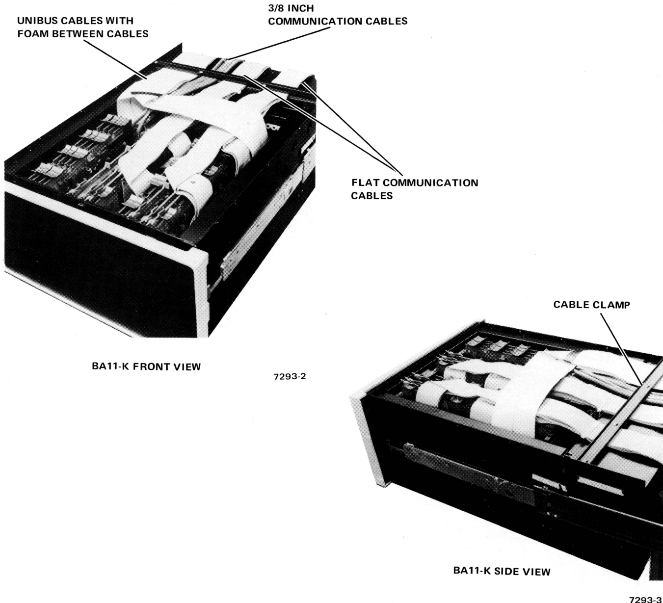
Figure 2-5 Cable Routing
