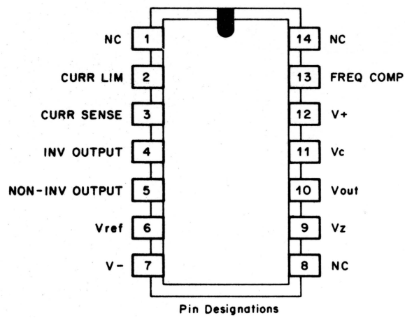
Figure 3-9 Voltage Regulator E1, Simplified Diagram
